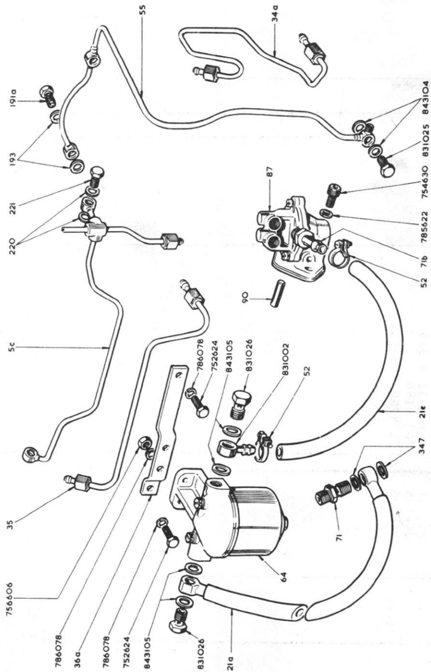
PLATE E FUEL PUMP, FILTER AND PIPES
