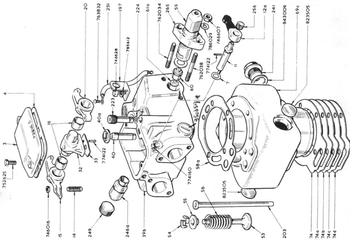
PLATE B CYLINDER AND CYLINDER HEAD
