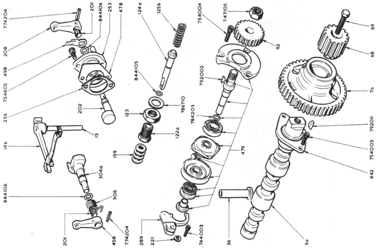
PLATE D CAMSHAFT, GOVERNOR AND CONTROLS
